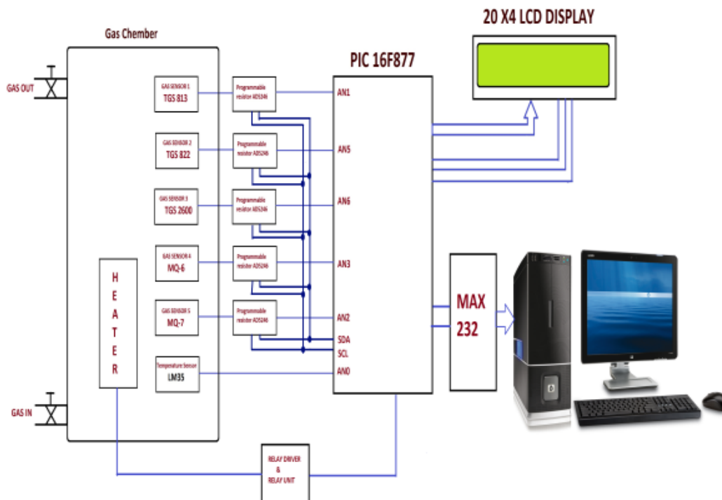
Fig. (2) The block diagram of hardware implementation of gas sensing detector system
