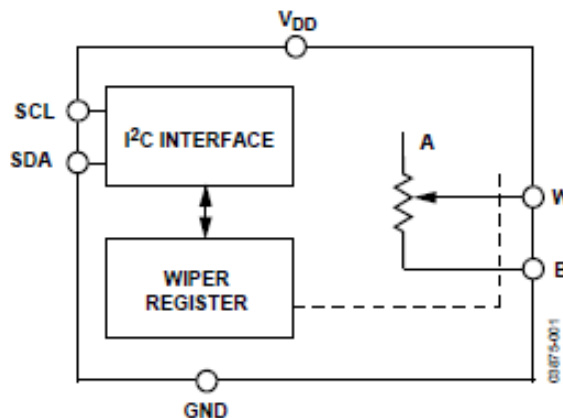
Fig. (4) Functional Block diagram of Programmable Resistor AD5246
