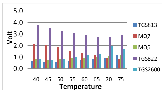
Figure 15: Sensors output for 1000 ppm Carbon monoxide gas at 4k load.
