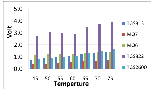
Figure 10: Sensors output for 100 ppm LPG gas at 4k load
