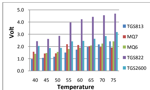
Figure 8: Sensors output for 400 ppm Methane gas at 4k load
