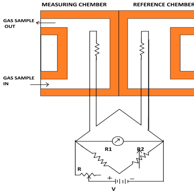
Fig. (1) Thermal conductivity Gas Analyzer circuit.
